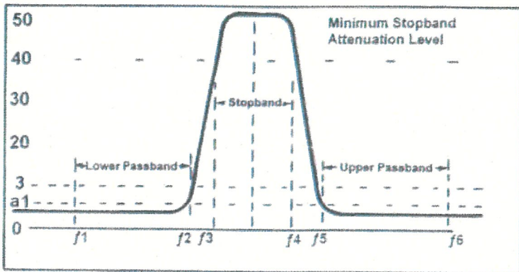
↑ ATTENUATION (dB) BAND REJECT
