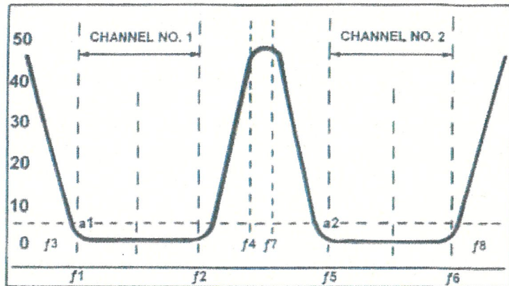
↑ ATTENUATION (dB) DIPLEXER Note required losses at each frequency
